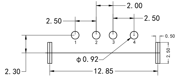
Recommended P.C.B Layout (±0.05)
